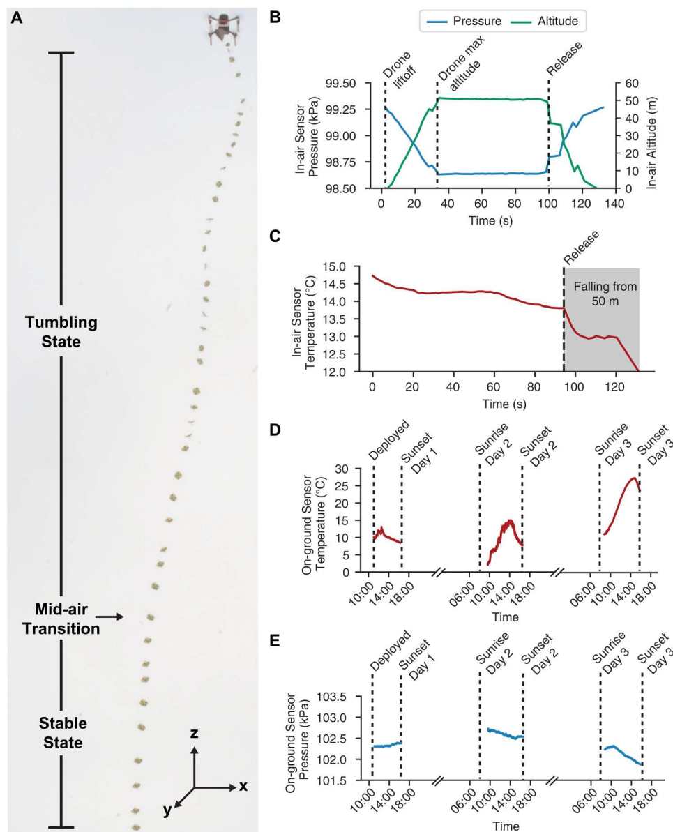
Fig. 7. In-air and on-ground microflier measurements. (A) Images showing our origami microflier falling from a drone and transitioning from its tumbling to stable state in mid-air. (B) Real-time pressure sensor readings sent via Bluetooth showing the altitude of our origami when dropped from 50 m. (C) Real-time temperature sensor readings sent via Bluetooth showing the temperature as our sensor falls. (D) Temperature readings from a 3-day outdoor deployment demonstrating that the microflier cold starts daily with harvested power. (E) Pressure readings from the 3-day outdoor deployment.
